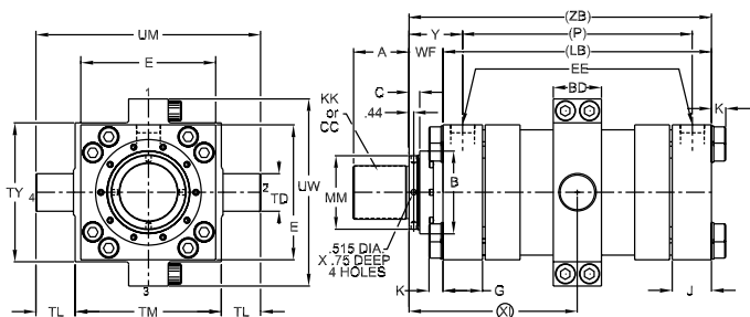
NFPA STYLE MT4 INTERMEDIATE FIXED TRUNNION MOUNTING
