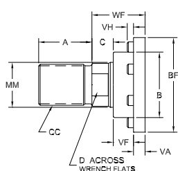
STYLE 2 Overize Male Thread
