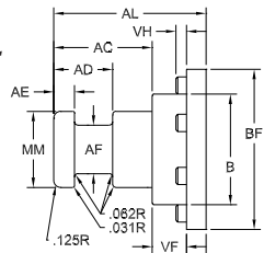
STYLE 5 Safety Coupler
