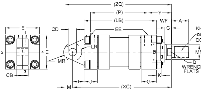
MH-PB-1 1.5" thru 8" Bore
