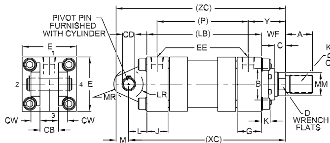
MH-SA* 1.5" thru 6" Bore
