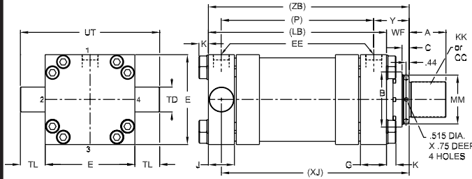
MH-TM-2 10" thru 14" Bore
