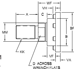
STYLE 1 Standard Male Thread
