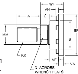
STYLE 4 "SPECIALS" THREAD STYLE 4
