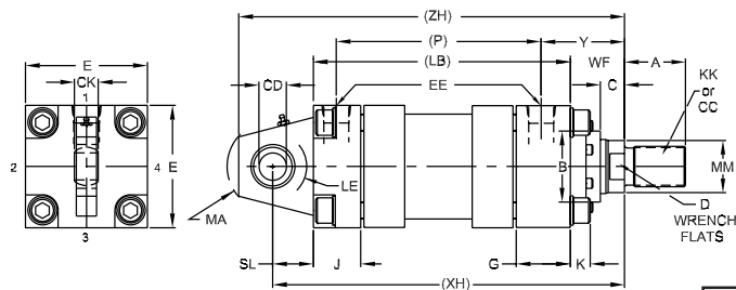
MH-SA* 1.5" thru 6" Bore
