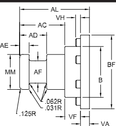
STYLE 5 Safety Coupler
