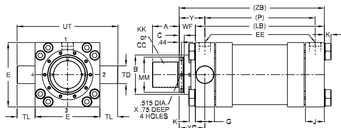
MH-TM-3 10" thru 14" Bore
