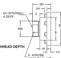
STYLE 3 Female Thread
